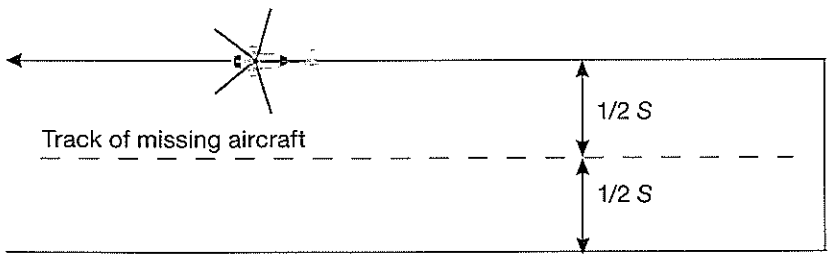
Track line search, return (TSR)
