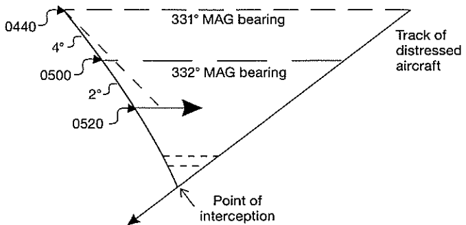
Offset or beam-on intercept: method 3
