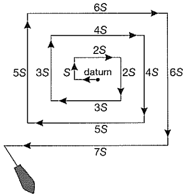
Expanding square search (SS)
