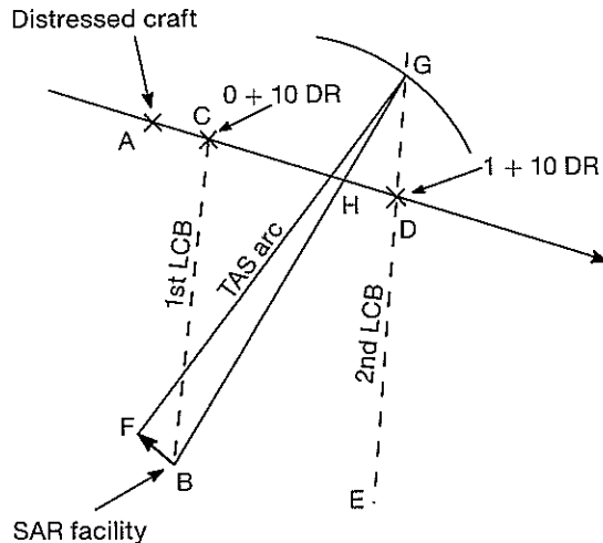
Offset or beam-on intercept: method 2
