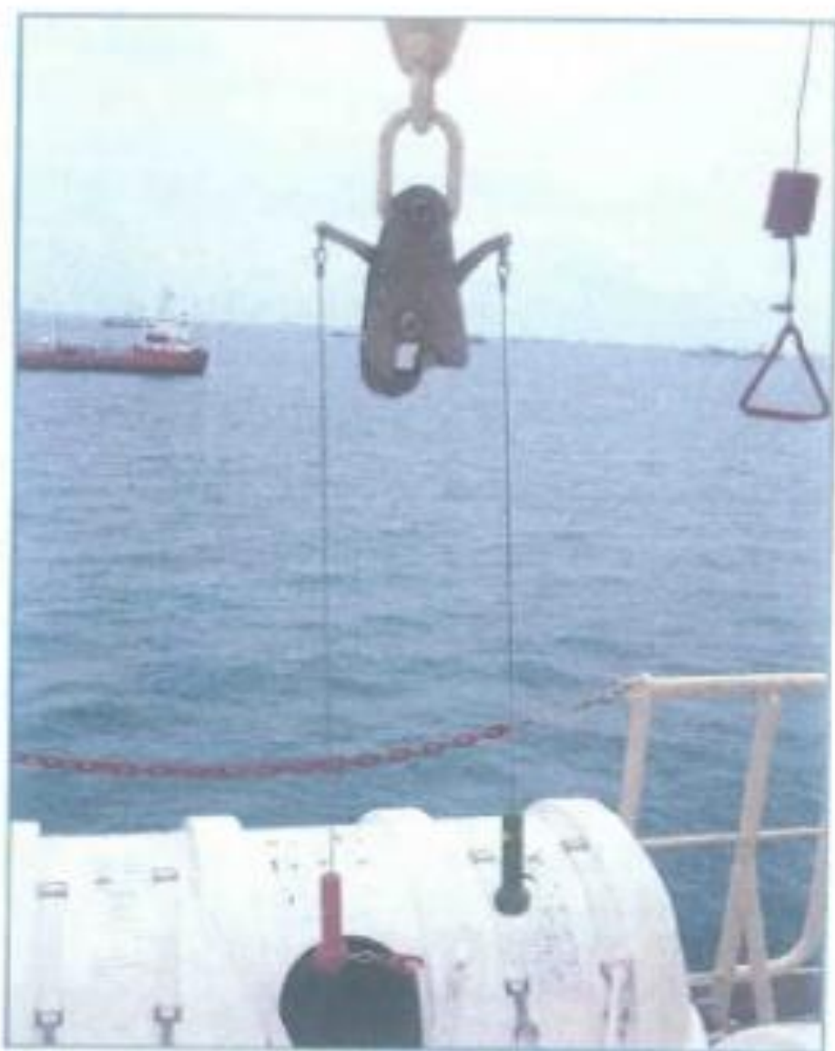
Fig. 12 Off-load release hook for davit launched liferaft
